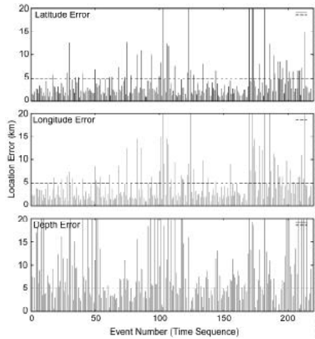
Figure 6. Location errors in latitude, longitude and depth (in km) for the Ghaen-Birjand 1997 aftershock sequence, after relocation with improved crustal model following the VELEST inversion.
