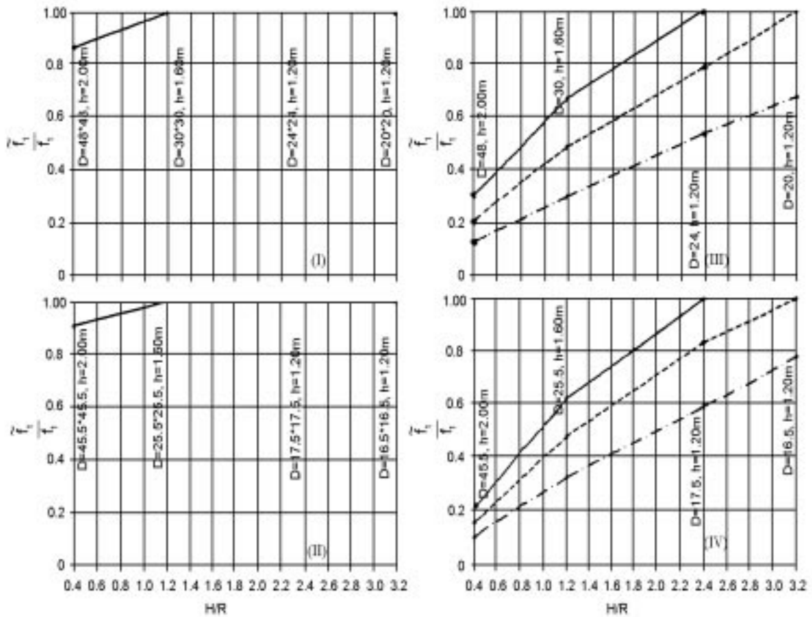
Figure 10. The effect of foundation thickness on the frequency ratio for various types of foundations located on medium soil.
