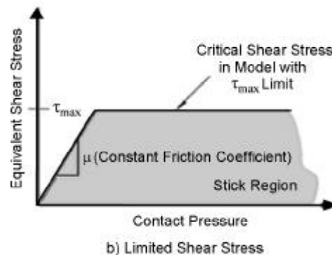
Figure 3. Slip regions for the friction model ( c = 0 ).
