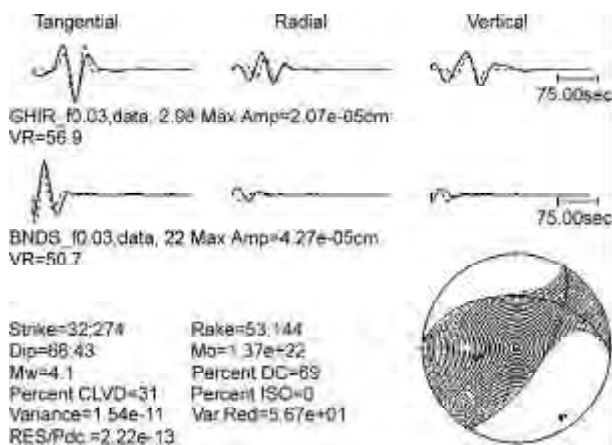
Figure 6. The result of modeling a minor aftershock with M_L = 4.1 as located by IIEES which have occurred on 06.06.03 at 07:14 origin time. Full waveform three components of BND5 (distance of 66km) and GHIR (distance of 320km) stations have been inverted and waveform fit is depicted. The data are shown as solid lines and the synthetics are dashed.
