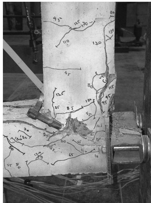
Figure 6. Pattern of cracking in the moment frame F1.
