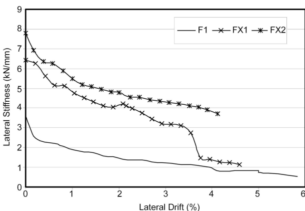
Figure 14. Degradation of the lateral stiffness of test frames.
