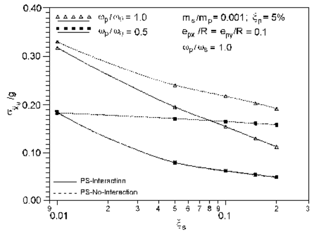
Figure 8. Variation of (\sigma_{\bar{x}_a} / g) with \xi_s for \omega_p / \omega_s = 1.0 .
