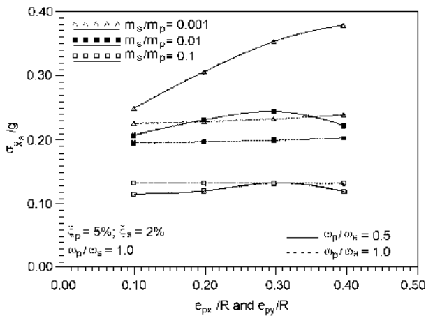
Figure 6. Variation of (\sigma_{\bar{x}_a} / g) with m_s / m_p for \omega_p / \omega_s = 1.0 .
